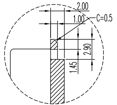
DETAIL B(3:1)
